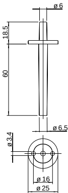
Climaset® 6555/6557
