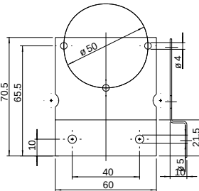
Mounting bracket 6402
