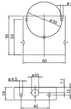
Mounting bracket 6401
