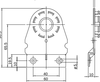
Mounting bracket 6401
