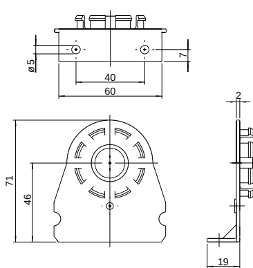
Mounting bracket 6482
